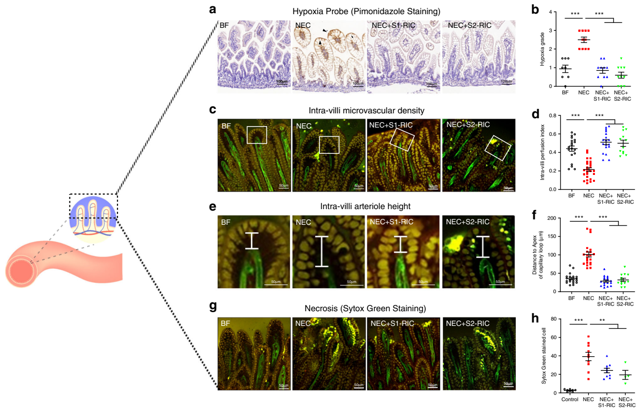
Fig. 5 RIC improves intestinal villi microvasculature and reduces ischemia and necrosis of enterocytes at the villi tip. a, b Pups were injected with pimonidazole, a sensitive marker which allows localization of intestinal ischemia. Data represent immunohistochemistry of pimonidazole in the ileum comparing breastfed (BF) control ( n = 8 ), NEC ( n = 10 ), NEC with Stage 1 RIC ( n = 10 ), and NEC with Stage 2 RIC ( n = 10 ). Scale bars are equivalent to 100 \mu\text{m} in the images shown. c Intra-villi microvasculature was investigated in Rosa MT/mG/+ ;Tie2-Cre using TPLSM and compared between BF, NEC, NEC with Stage 1 RIC, and NEC with Stage 2 RIC ( n = 4 per group; and minimum of 2 measurements were obtained per group). d Villus perfusion index was calculated as the ratio of the area of intra-villi arterioles to the area of the whole villi and compared between the listed groups. e, f The distance between the apex of the capillary loop and the apical side of the villi epithelium was measured and compared between listed groups. g Cell death (yellow staining in the tip of villi) in the ileal epithelium was detected using Sytox Green, a marker of necrosis which does not permeate into live cells but binds to cellular nucleic acids in dead cells, staining them with intense green fluorescence and was compared between listed groups. h Necrotic cells were counted in the listed groups ( *p < 0.05 ; **p < 0.01 ; ***p < 0.0001 ). Data were compared using two-sided one-way ANOVA with post hoc Turkey test ( **p < 0.01 ; ***p < 0.0001 ). Scale bars in (c, e and g) are equivalent to 50 \mu\text{m} , and data are presented as mean \pm SEM. Source data are provided as a Source Data file.
